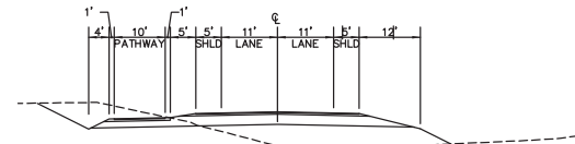
FRONTAGE ROAD W/PATHWAY
