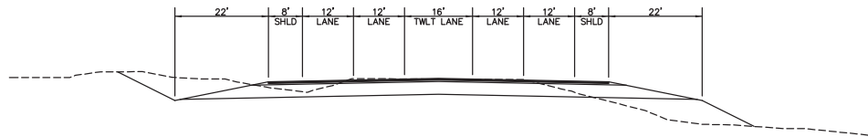
PARKS HIGHWAY 5-LANE SECTION LUCUS RD TO CHURCH RD
