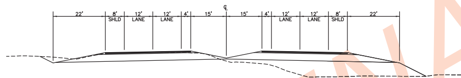
PARKS HIGHWAY 4-LANE DIVIDED MEDIAN SECTION CHURCH RD TO MUSEUM RD
