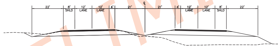
PARKS HIGHWAY 4-LANE DIVIDED MEDIAN SECTION MUSEUM RD TO BIG LAKE RD
