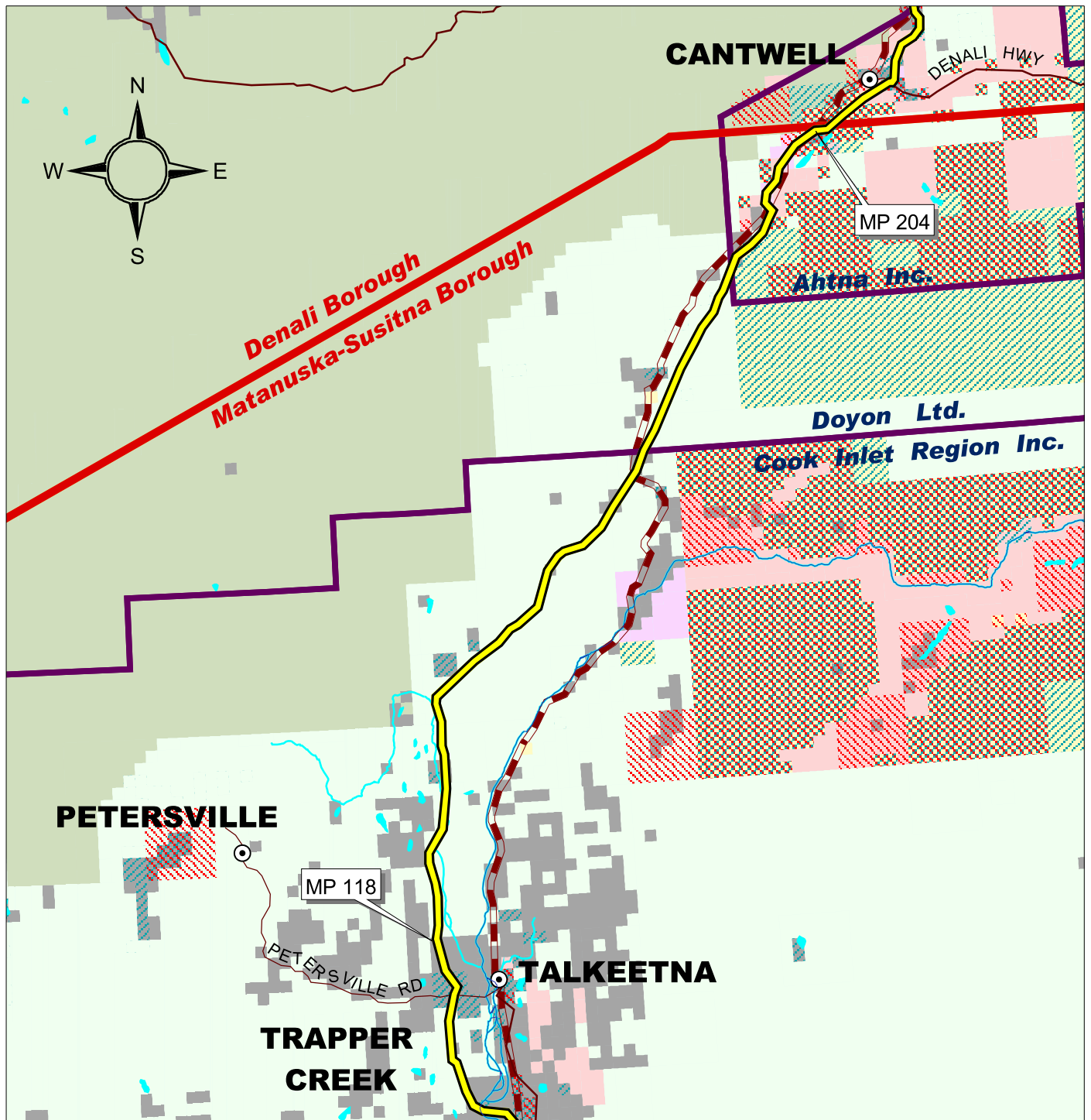
Figure 4-15 Parks Highway Trapper Creek to Broad Pass MP 118 to 204
